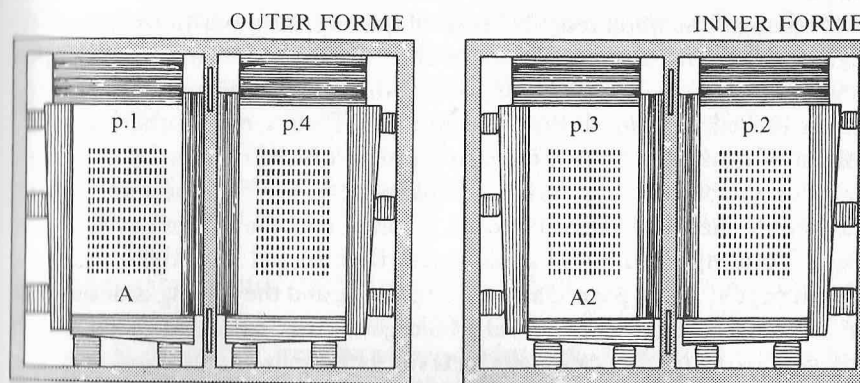
FIG. 44. The two formes for a sheet of folio, showing the disposition of the pages (cf. fig. 46). The furniture is so arranged that the head-, side-, foot-, and gutter-sticks will not bind on each other when the quoins are driven up tight. The cross of the chase has slots in it to protect the points of the press when the tympan is folded down.
